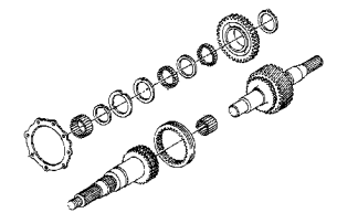
244-400 Gear Train
